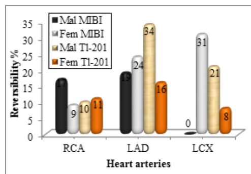
Figure 3: shows the reversibility% of ischemic disease in coronary arteries (Left Anterior descending (LAD) Right coronary artery (RCA) Left Circumflex (LCX) using ^{99\text{m}}\text{Tc} -MIBI & ^{201}\text{Tl} , (M = mala, F = female).
