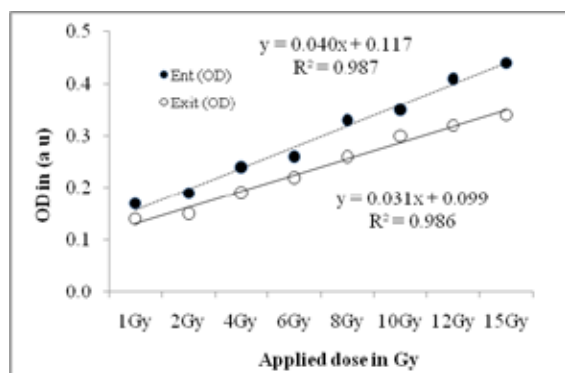
Figure 5 shows the correlation between dose in Gy and the relevant optical density in (a. u).
