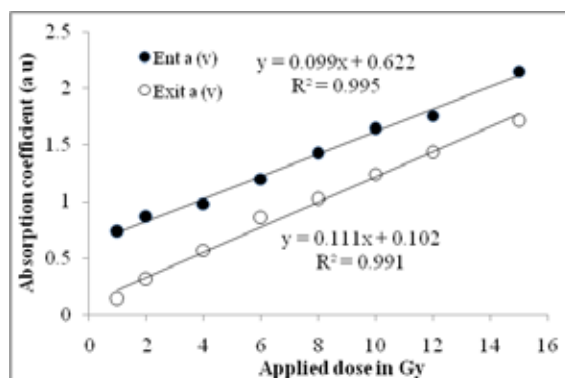
Figure 4 shows the correlation between the applied g-radiation doses 1-15 Gy and the absorption coefficient at entrance and exit doses.
